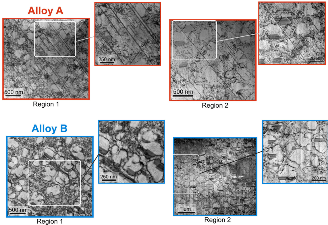
Fig. 6—STEM micrographs of the deformation structures observed for both alloys after testing at 760 °C and 552 MPa. Micrographs are taken from samples extracted from (001) grains oriented perpendicular to (011) crystal orientation. Overall and detailed micrographs are presented for both alloys.
