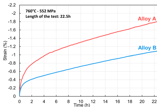
Fig. 4—Experimental creep curves for both Ni-based superalloys tested at 760 °C and 552 MPa. Creep tests were stopped at 22.5 hours.
