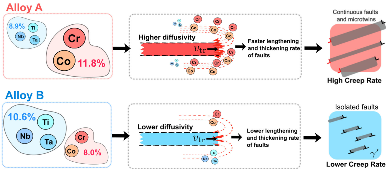
Fig. 14—Diagram of the influence of the alloy composition on the lengthening process of segregation-assisted fault and its connections with the observed operative deformation mechanisms.
