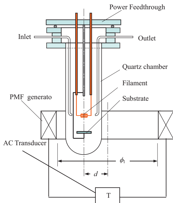
Fig. 1. Schematic diagram of the periodic magnetic field HFCVD system.
