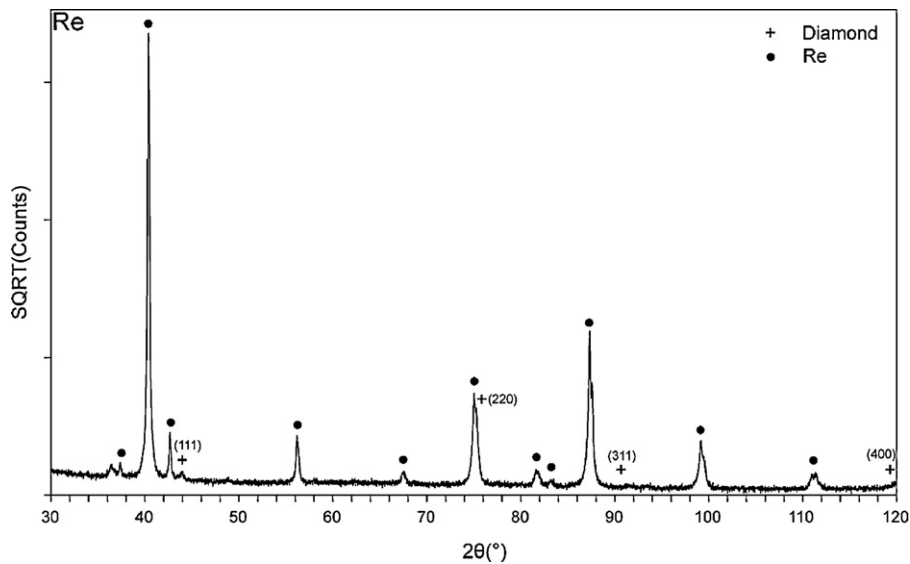
Fig. 3. X-ray diffraction patterns of diamond films deposited on Re substrate.
