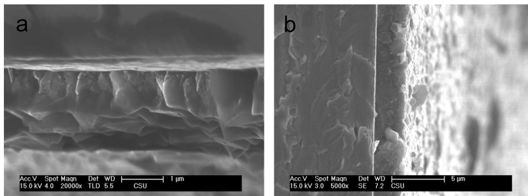
Fig. 2. The cross-section SEM image of diamond films grown at methane concentrations of 1%. (a) Without the PMF and (b) \omega = 30,000 rpm under the PMF.
