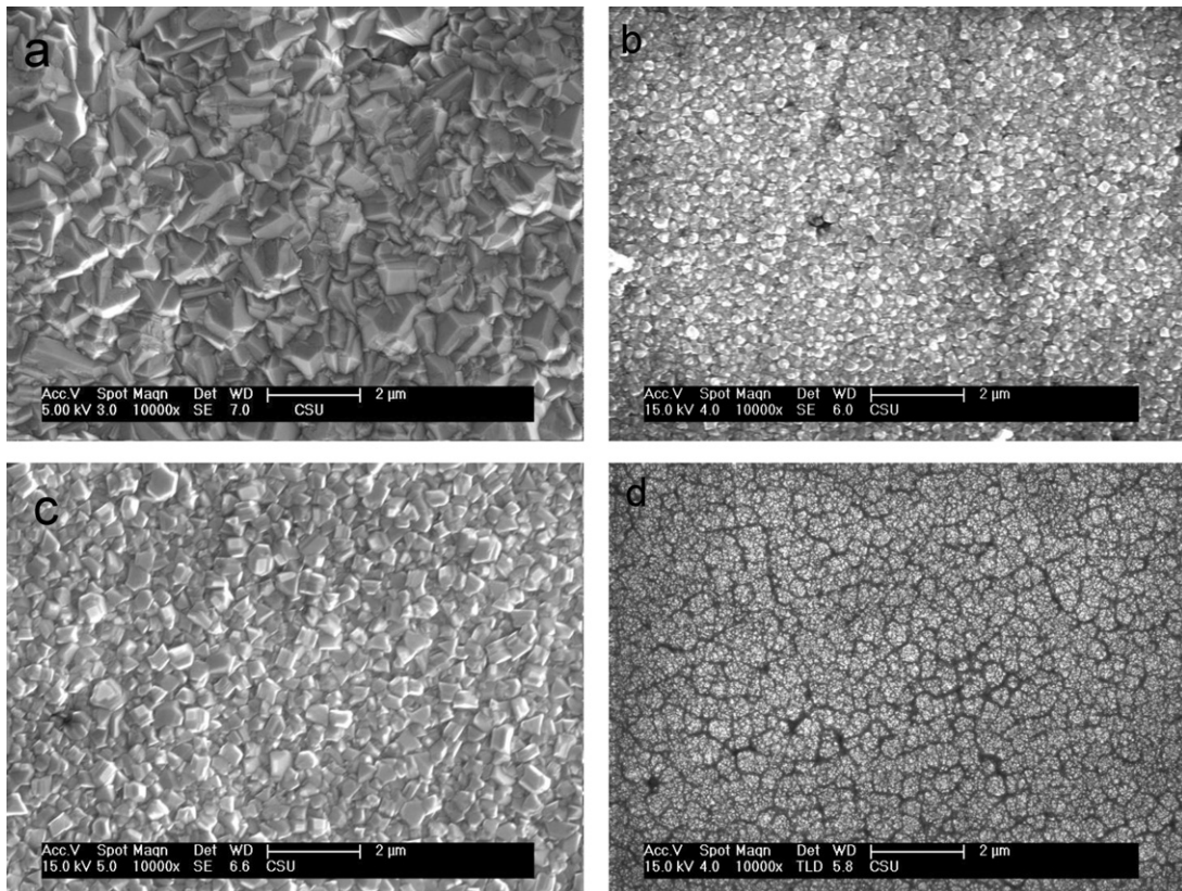
Fig. 4. The SEM images of diamond films in different doped concentrations: (a) 0.5% (without the PMF), (b) 0.5% ( \omega = 30,000 rpm under the PMF), (c) 2% (without the PMF) and (d) 2% ( \omega = 30,000 rpm under the PMF).
