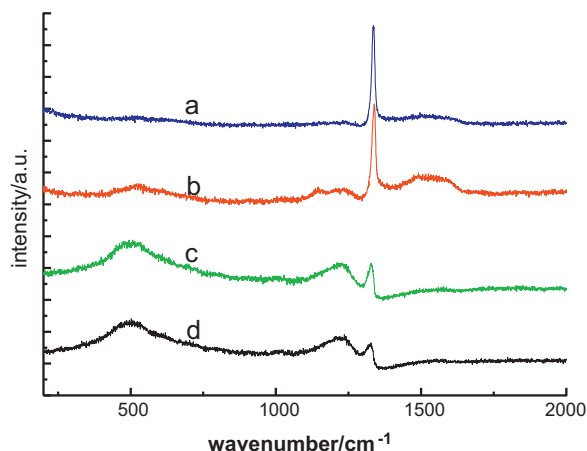
Fig. 5. Raman spectrum for the diamond films in different doped concentrations: (a) 0.5% (without the PMF), (b) 0.5% ( \omega = 30,000 rpm under the PMF), (c) 2% (without the PMF) and (d) 2% ( \omega = 30,000 rpm under the PMF).
