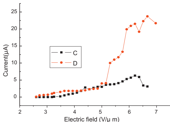
Fig. 6. Characteristics of field emission of the diamond film.
